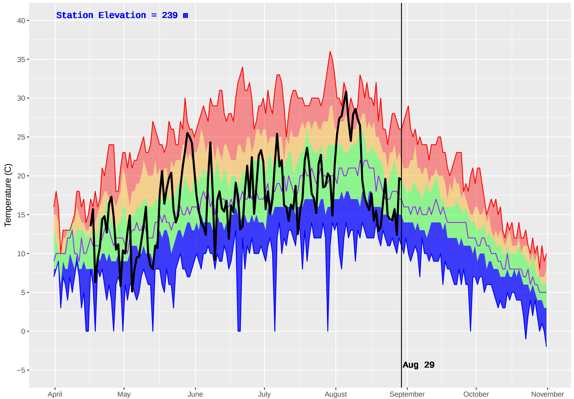
ROSSWOOD (105) : Historical (1970–2016) and Current (2017) Noon Temperature
