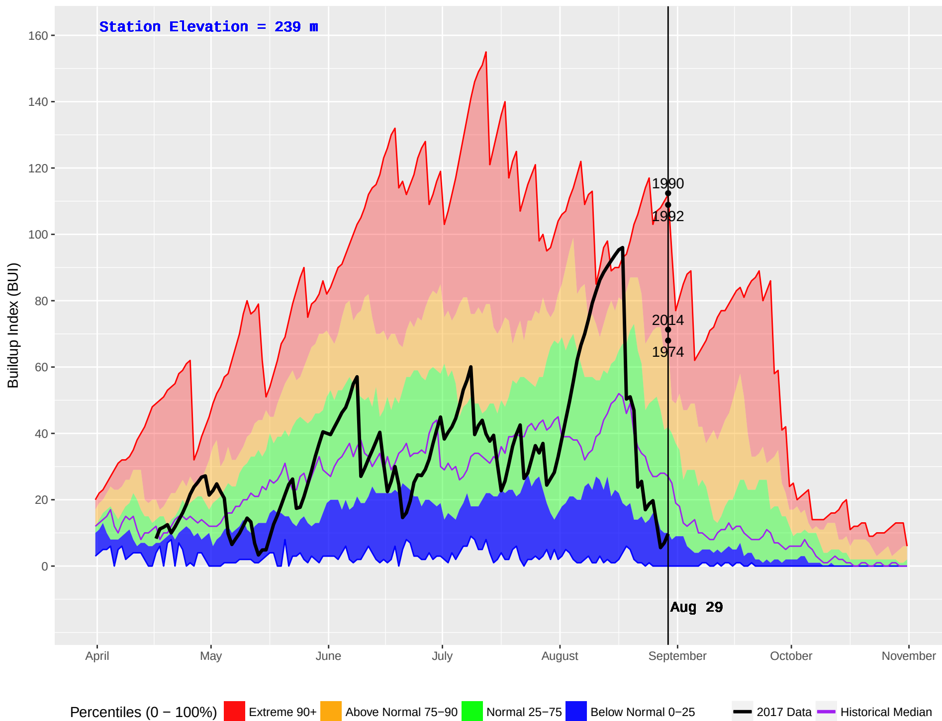
ROSSWOOD (105) : Historical (1970–2016) and Current (2017) Noon Buildup Index (BUI)
